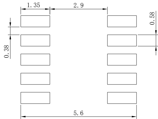
Soldering Patterns
